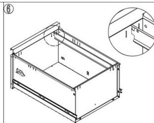
Fix the hanging rods with drawer panels as show in the picture.
